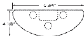
End View: Pendant Linear Direct/Indirect T8 3-Light.
