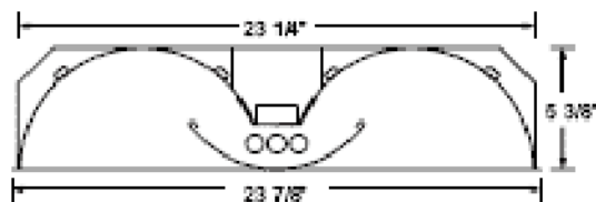
End View: 2x4 Recessed Deep Direct/Indirect
